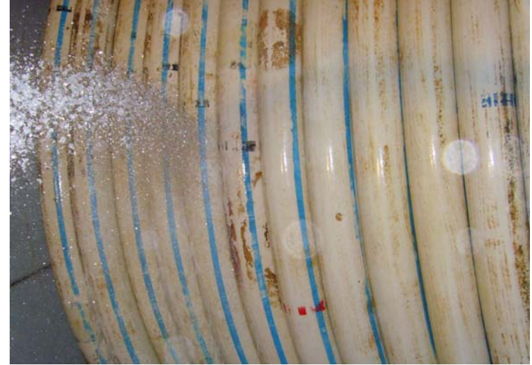
Riser external sheath condition following water jetting
